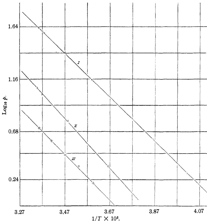
Fig. 5.—Vapor pressure curves of cyclobutanone (Curve I), cyclopentanone (Curve II) and cyclohexanone (Curve III, Radalescu).
